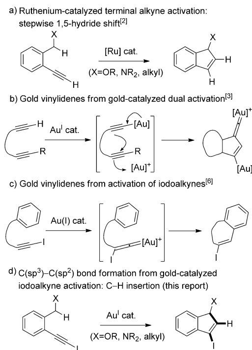
Scheme 1. Basis for the proposed \text{C}(\text{sp}^3)\text{--H} bond activation triggered by iodovinylidene generation from gold-catalyzed iodoalkyne isomerization.
